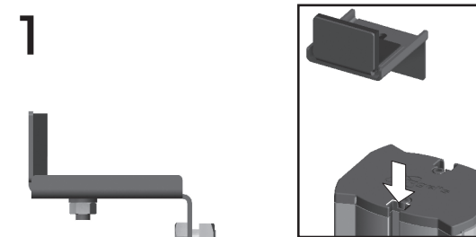
PFA 9127 Accessory clamp
